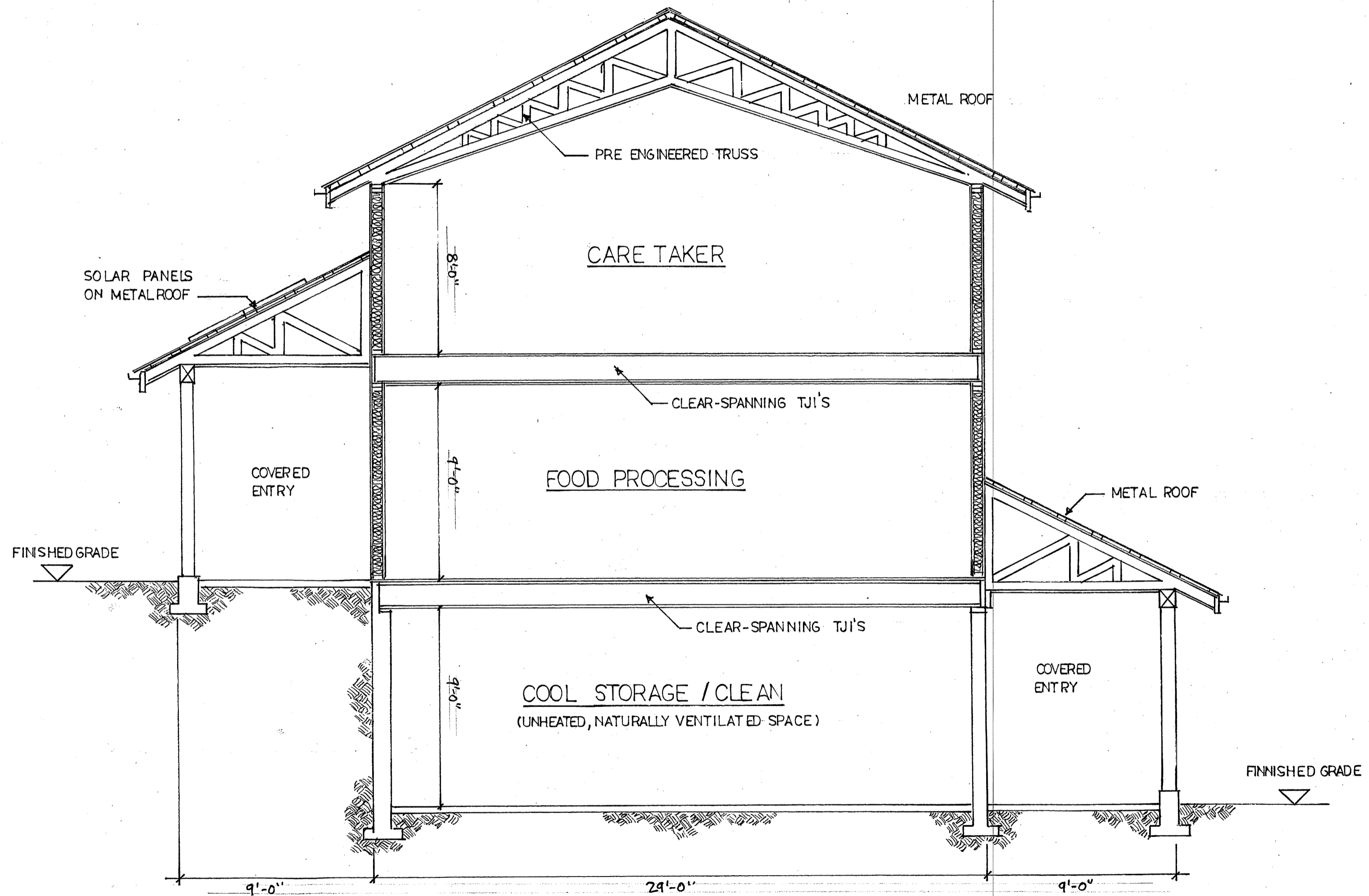
TYPICAL SECTION THROUGH BUILDING
